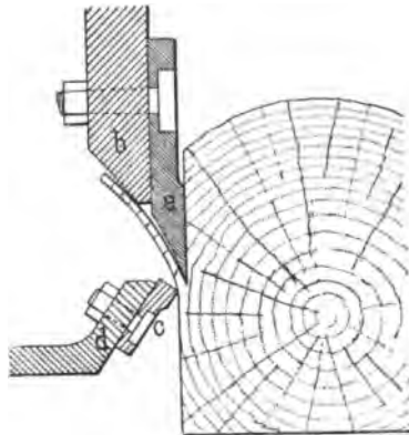
Fig. 305.—Plessis' machine.
